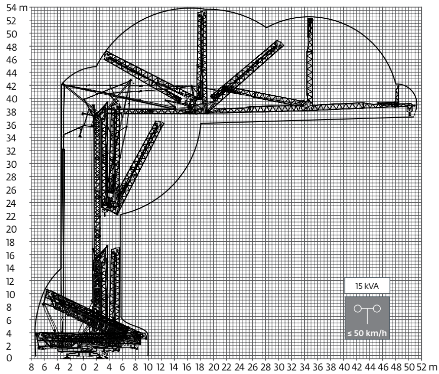
Jib raised 30°
