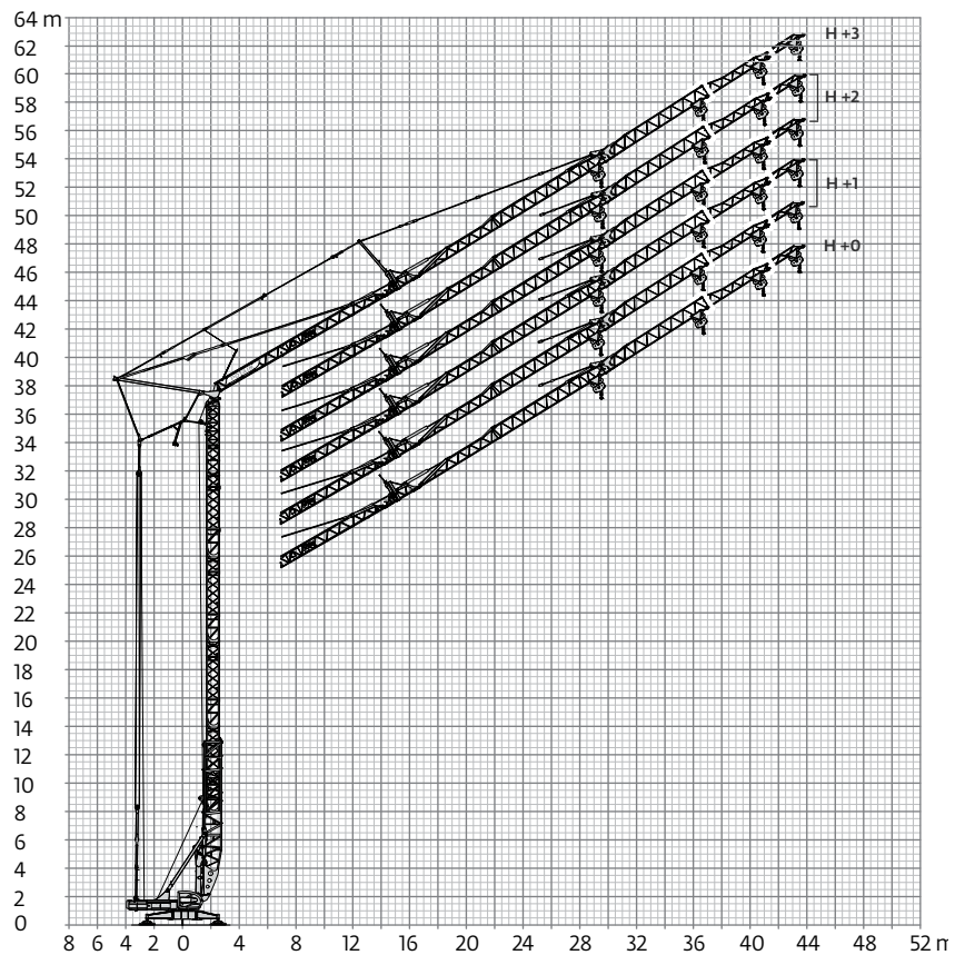
Jib raised 30°
