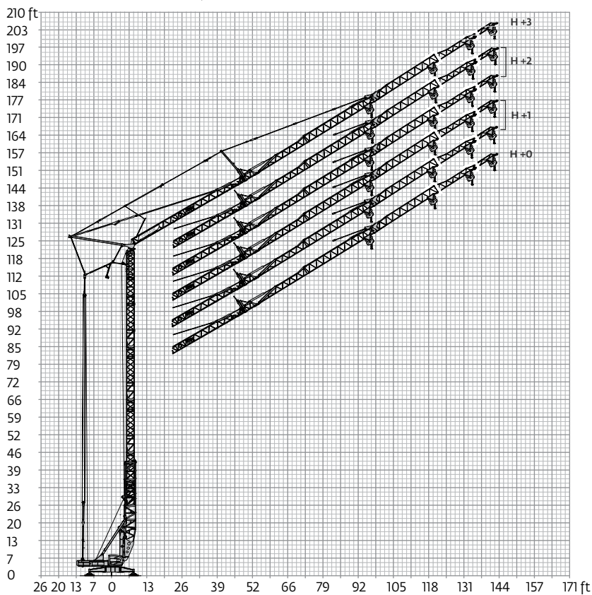
Jib raised 30°
